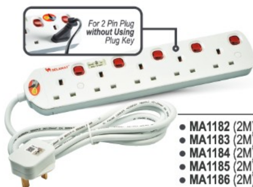
Portable Switched Socket Outlet with Individual Neon Switch
